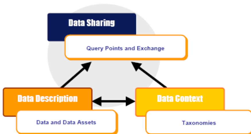
Figure 5: DRM Structure
