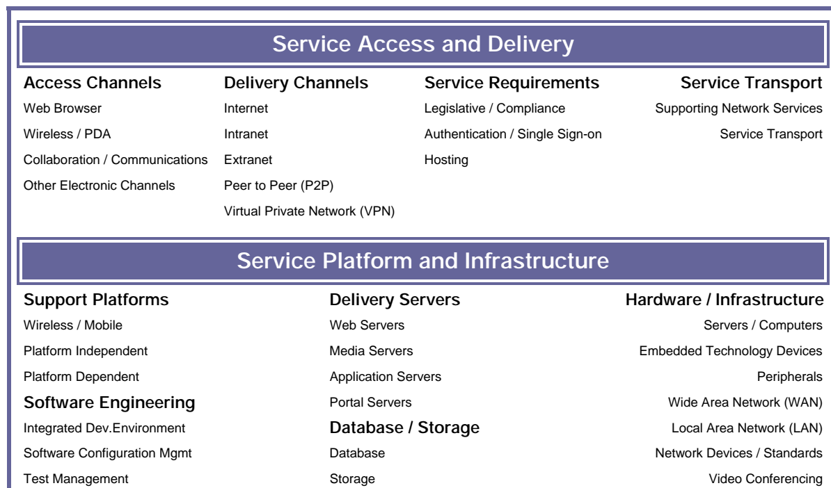
Figure 23: TRM Overview
