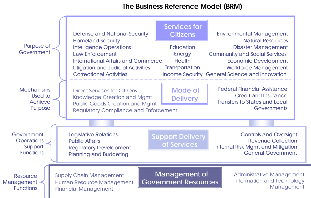
Figure 10: BRM Overview
