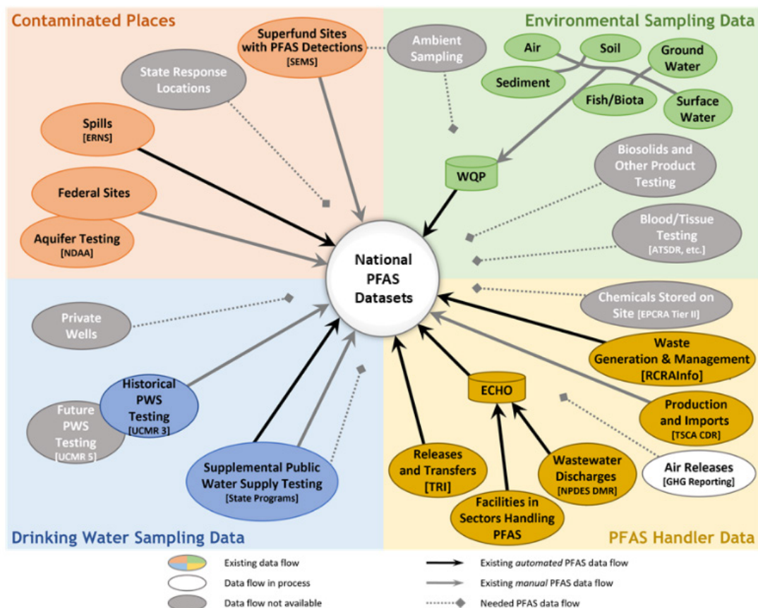
Figure 2: Available National (and Some State Level) Data on PFAS Sources and Environmental Occurrence 33 . WQP = Water Quality Portal; PWS = Public water system; ERNS = Emergency Response Notification System, UCMR = Unregulated Contaminant Monitoring Rule, NPDES = National Pollutant Discharge Elimination System, DMR = Discharge Monitoring Reports, RCRA = Resource Conservation and Recovery Act, SEMS = Superfund Enterprise Management System, TSCA = Toxic Substances Control Act, CDR = Chemical Data Reporting, NDA = National Defense Authorization Act, GHG = Greenhouse Gas, TRI = Toxic Release Inventory, ECHO = Enforcement and Compliance History Online (source: https://echo.epa.gov/tools/data-downloads/national-pfas-datasets )
