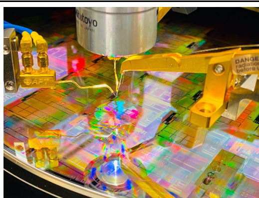
Integrated photonic devices in a probe station undergoing simultaneous optical and electronic measurement. Image credit: NIST.
